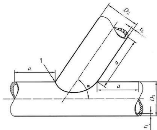
Fig. 6.3.1.6 Test piece for a branch connection:
