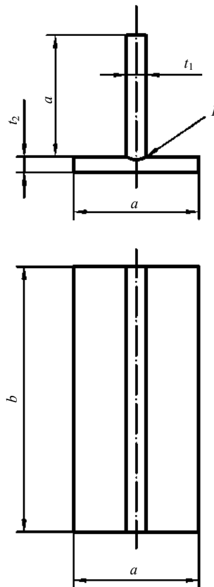
Fig. 8.2.2.6 Test piece for a tee-joint in plate and semi-finished product: l — edge preparation and fit-up as detailed in pWPS; t — base metal thickness; a \geq \text{mm} ; b \geq 350 \text{ mm}
