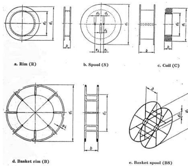
Fig. 5.3.3.3.3 Types of welding wire winding for supply: a — rim (R); b — spool (S); c — square-sectioned coil (C); d — basket rim (B); e — basket spool (BS)
